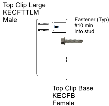
TOP CLIP LARGE AND BASE ASSEMBLY
