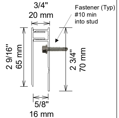
TOP CLIP LARGE AND BASE ASSEMBLED
