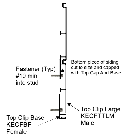
TOP DOWN- BOTTOM DETAIL
