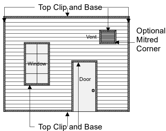
TOP CLIP LARGE AND BASE APPLICATIONS
